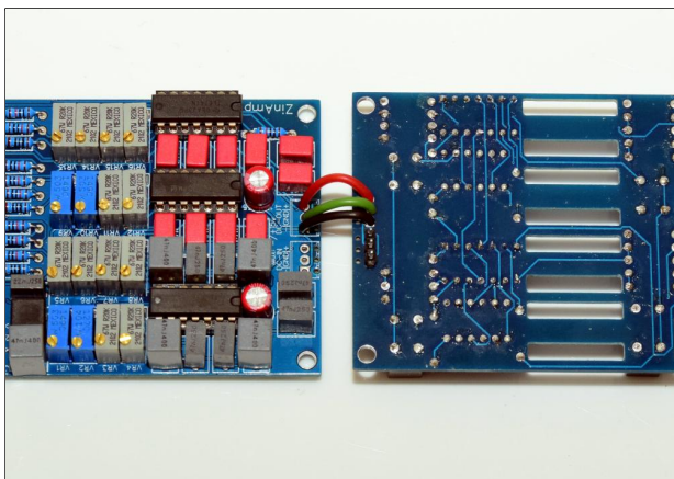
Power Connections
